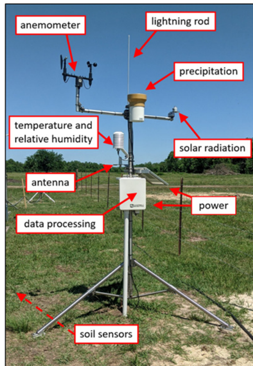
Figure 2. Soil water content monitoring station with additional meteorological monitoring equipment located in Guy, Texas. Dashed arrow indicates orientation of buried sensors relative to tower.
